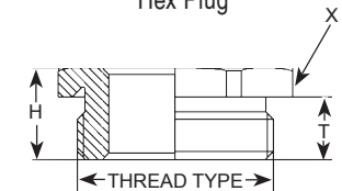
Nickel Plated Brass Hex Plug
